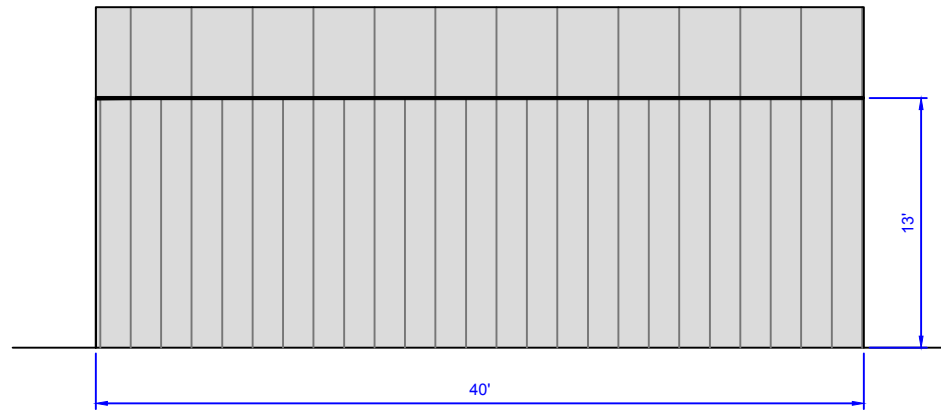
SIDES ELEVATION
