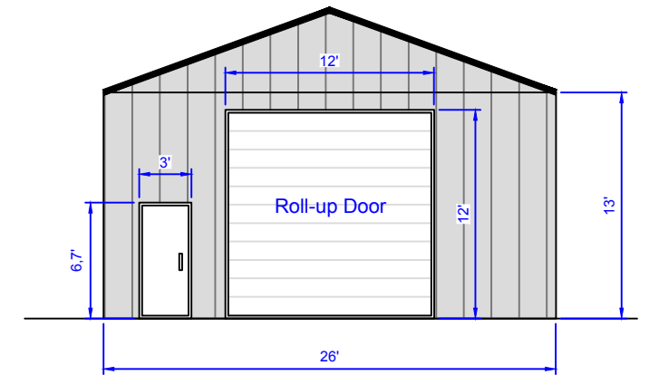
BACK ELEVATION
